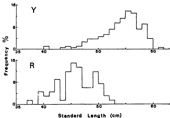
Fig. 4 Body length frequency histogram of two types of Pristipomoides typus caught in areas A and B by changi.
