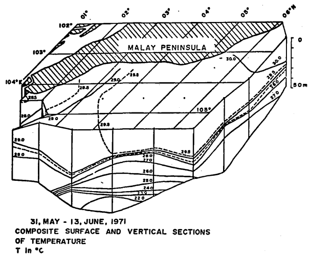
Fig. 3 Composite surface and vertical sections of temperature. May to June, 1971.
