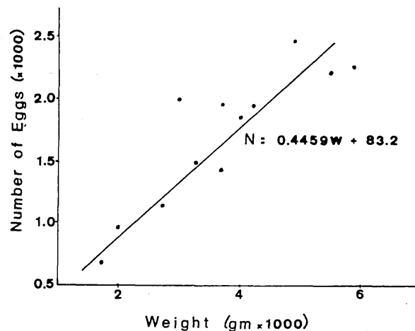
Fig. 8 Relationship between number of eggs ( \times 10^3 ) and fish weight (grams).
